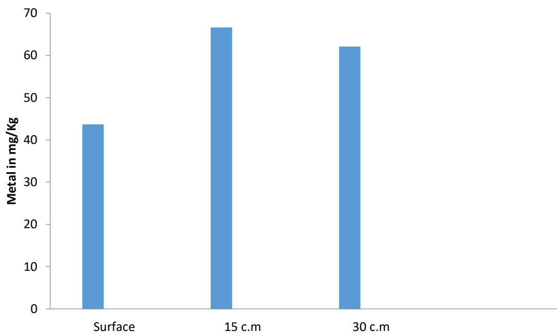
Fig:4 Chromium(Cr)
