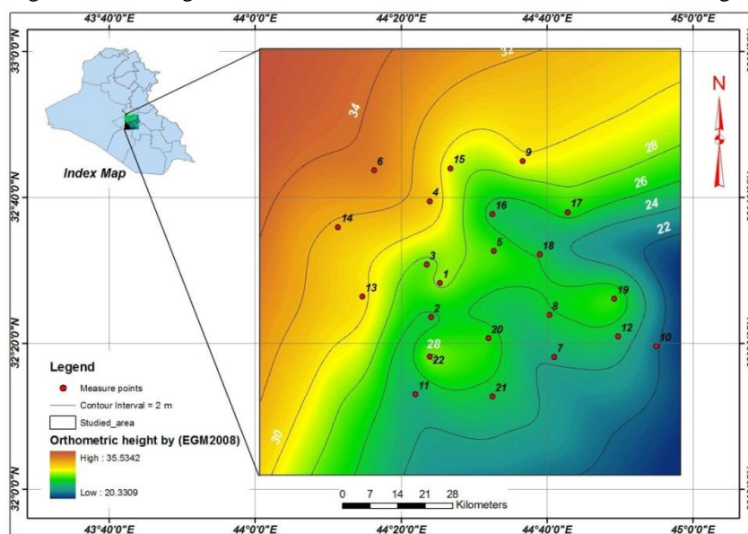
Figure 7: Contour map for orthometric height GPS data.
