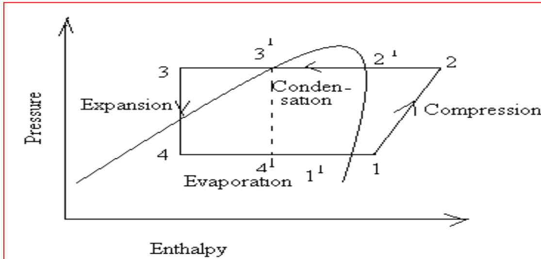
Fig. 3 P-h Plot with Sub-Cooling and super heating
