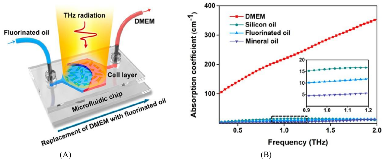
Fig. 7. Implementation of THz spectroscopy on living cells with a microfluidic platform (Yang et al., 2019). In (A), the platform is shown with two COP layers as THz windows bonded to a 100- \mu\text{m} -thick PET layer with 200- \mu\text{m} -wide microchannels. It is shown with fluorinated oil in its inlet, a hexagonal detection area, and an outlet for the Dulbecco's modified Eagle's medium (DMEM). In (B), results for the absorption coefficient versus frequency are shown for the DMEM, silicon oil, fluorinated oil, and mineral oil. The figure is reprinted (slightly modified) with permission from (Yang et al., 2019). Copyright (2019) American Chemical Society.
