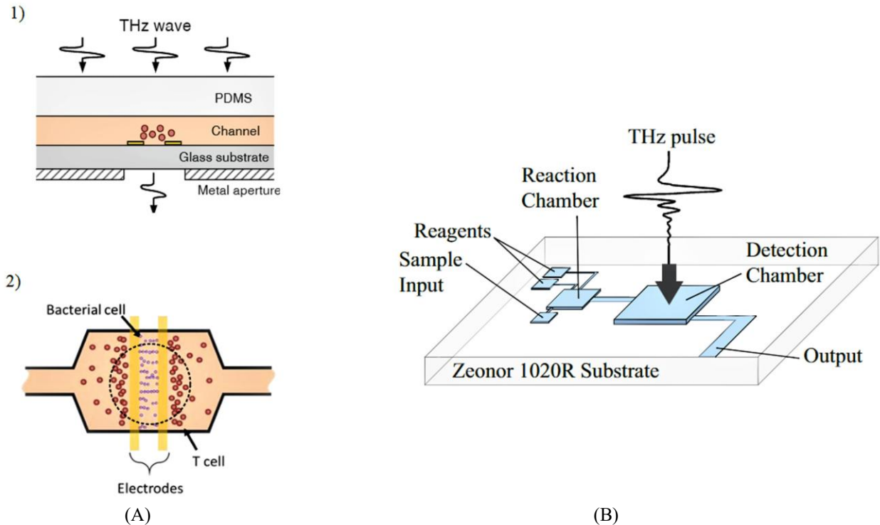
Fig. 5. Examples of THz-microfluidic platforms based upon polymeric materials. In (A), a PDMS-based THz-microfluidic platform is shown. Diagram 1) shows its glass substrate, PDMS layer with a 300- \mu\text{m} -thick channel, and two gold electrodes, between which cells are trapped. Diagram 2) shows a top view of the microfluidic platform after applying voltage to the electrodes. This figure is reprinted (with a slight modification) from (Tang et al., 2016). In (B), a COP-based THz-microfluidic platform is shown. It consists of a sample input, reagents, a reaction chamber to react the sample with the reagents, a detection chamber in which THz radiation is passed through, and the output. This figure is reprinted with permission from (George et al., 2008) © The Optical Society.
